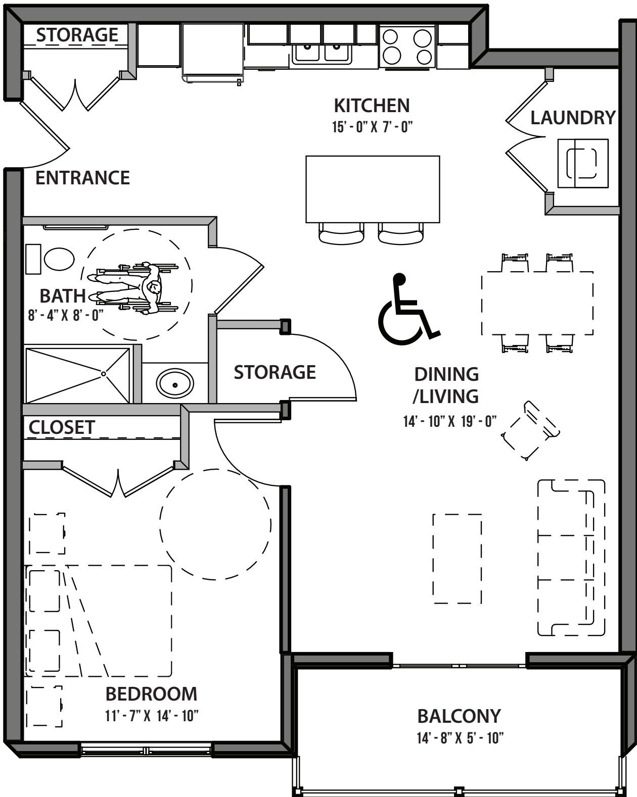
1 BEDROOM BARRIER FREE SUITE SUITE F - 800 SQ FT + BALCONY
