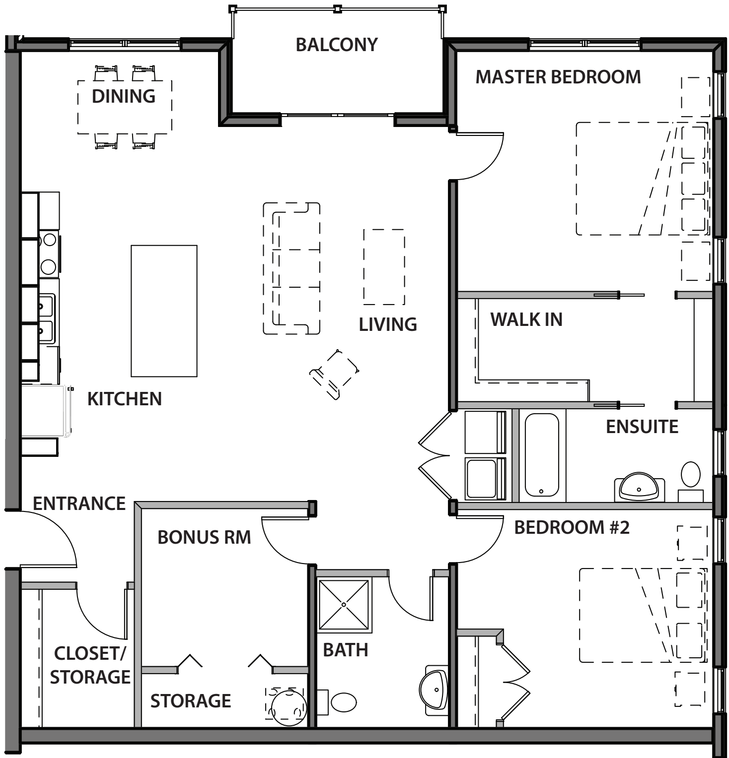
2 BEDROOM SUITE - WITH ENSUITE SUITE C - 1280 SQ FT + BALCONY
